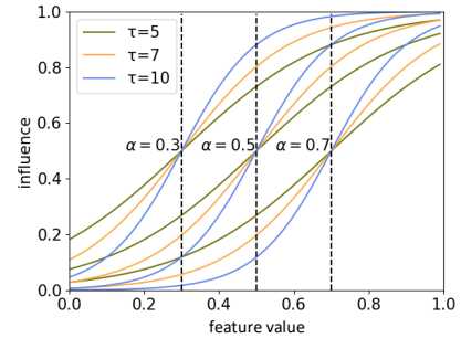
Fig. 4. the Examples of Sigmoid Function.
