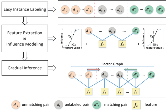
Fig. 2. Paradigm Overview.
