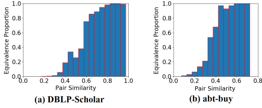
Fig. 3. Empirical Validation of the Monotonicity Assumption.
