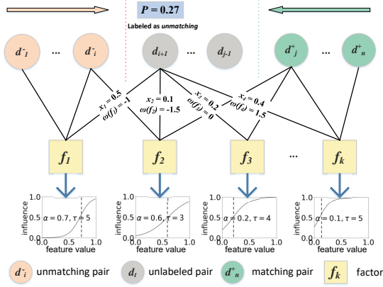
Fig. 5. An Example of Factor Graph.
